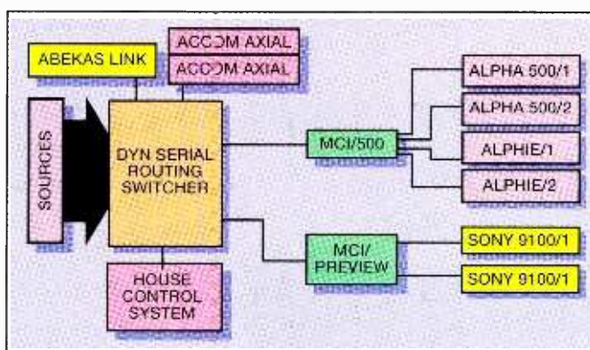
Figure 4. Block diagram illustrating the power of the Alpha Image control system. Using multiple control interfaces (MCIs), the system can be used to feed several switchers.
